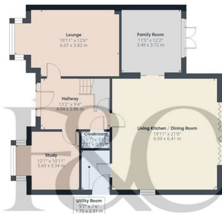
Floor 0 Building 1
